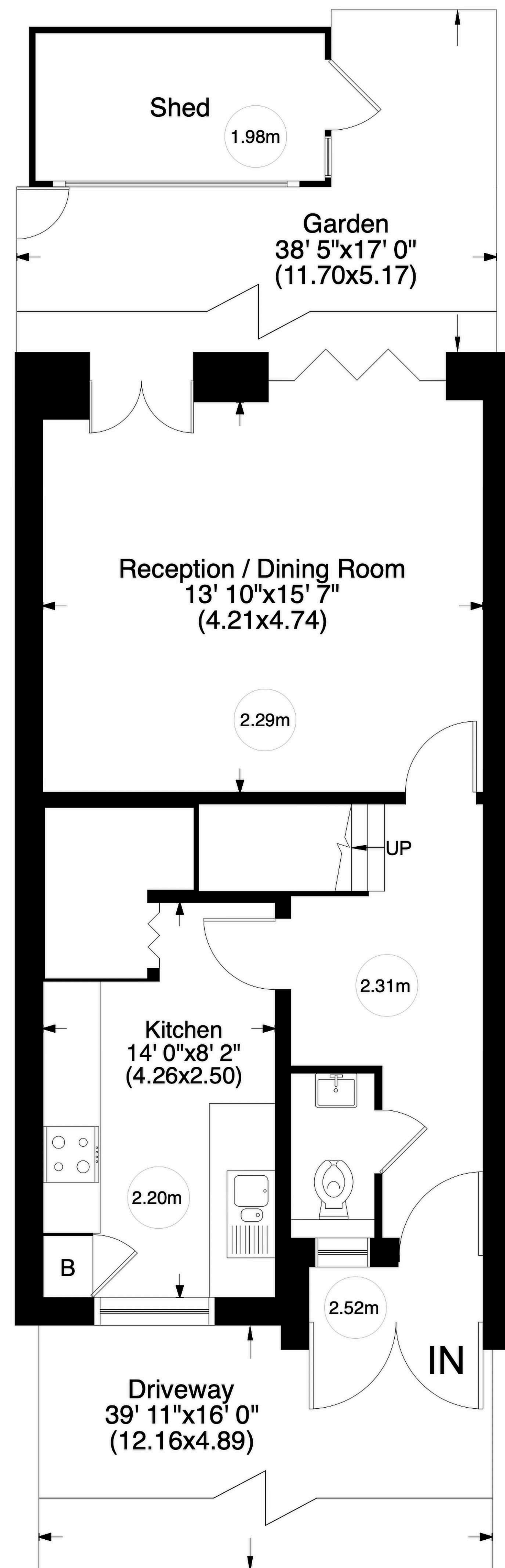
Ground Floor
