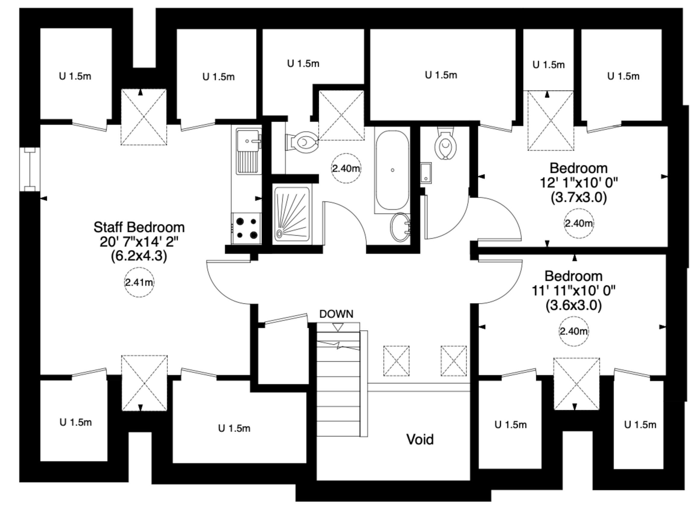
First floor
