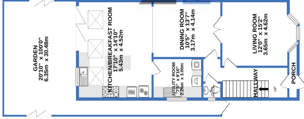
GROUND FLOOR 770 sq.ft. (71.5 sq.m.) approx.
